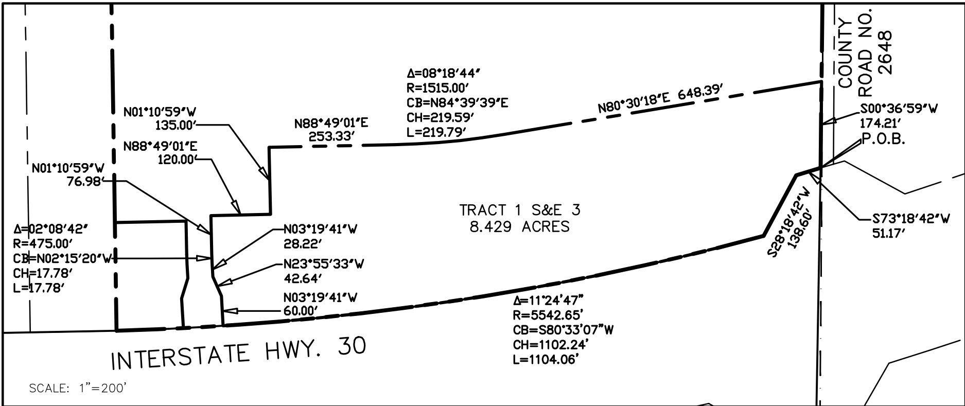
DETAIL "C"
